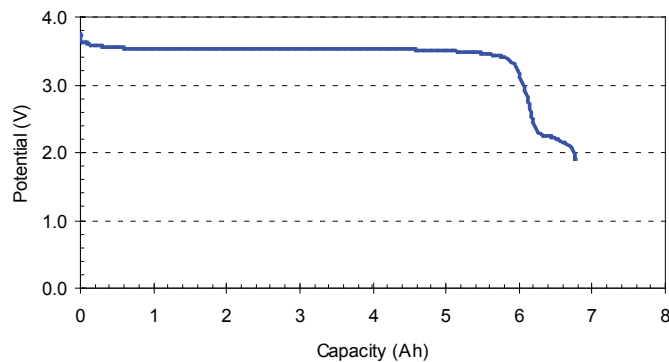
Discharge at 30 mA, 150°C
